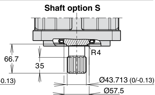
Type S spline shaft SAE J498b, class 1; 30° involute spline; 13T-8/16 DP; flat root, side fit
