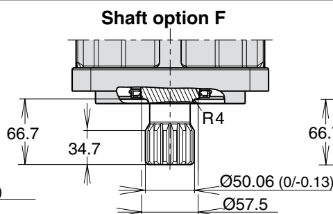
Type F spline shaft SAE J498b, class 1; 15T-8/16 DP; fillet root, side fit
